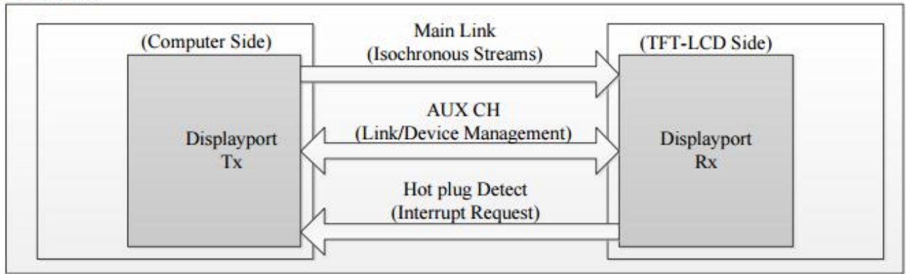
Fig.4-2-1 DP architecture
